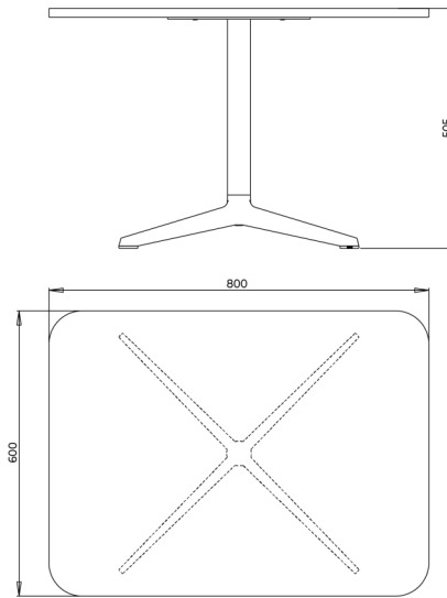
800x600x505 - 4 star
