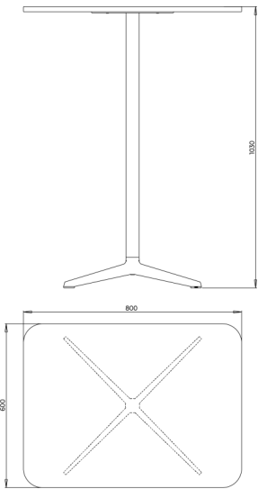
800x600x1030 - 4 star
