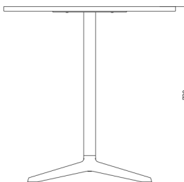
Ø700x720 - 4 star
