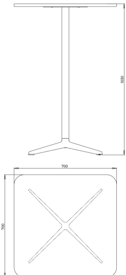
700x700x1030 - 4 star
